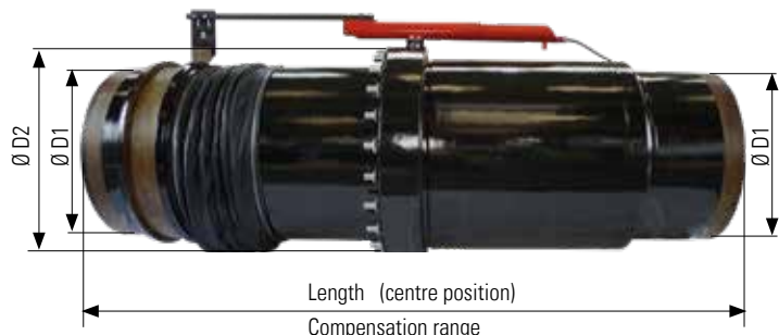
Without pressure testing locking system (Compensator in centre position)
