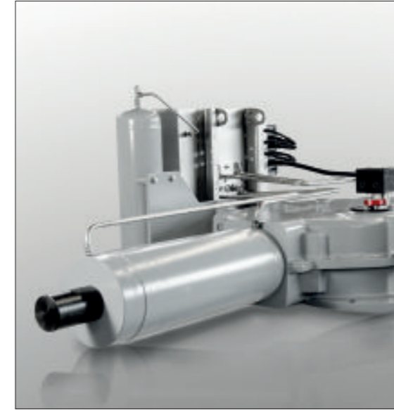
Right: Type KY control with remote control OPEN/CLOSE, incl. - Torque limitation - Automatic pipe fracture response with manual reset and optional adjustment set
