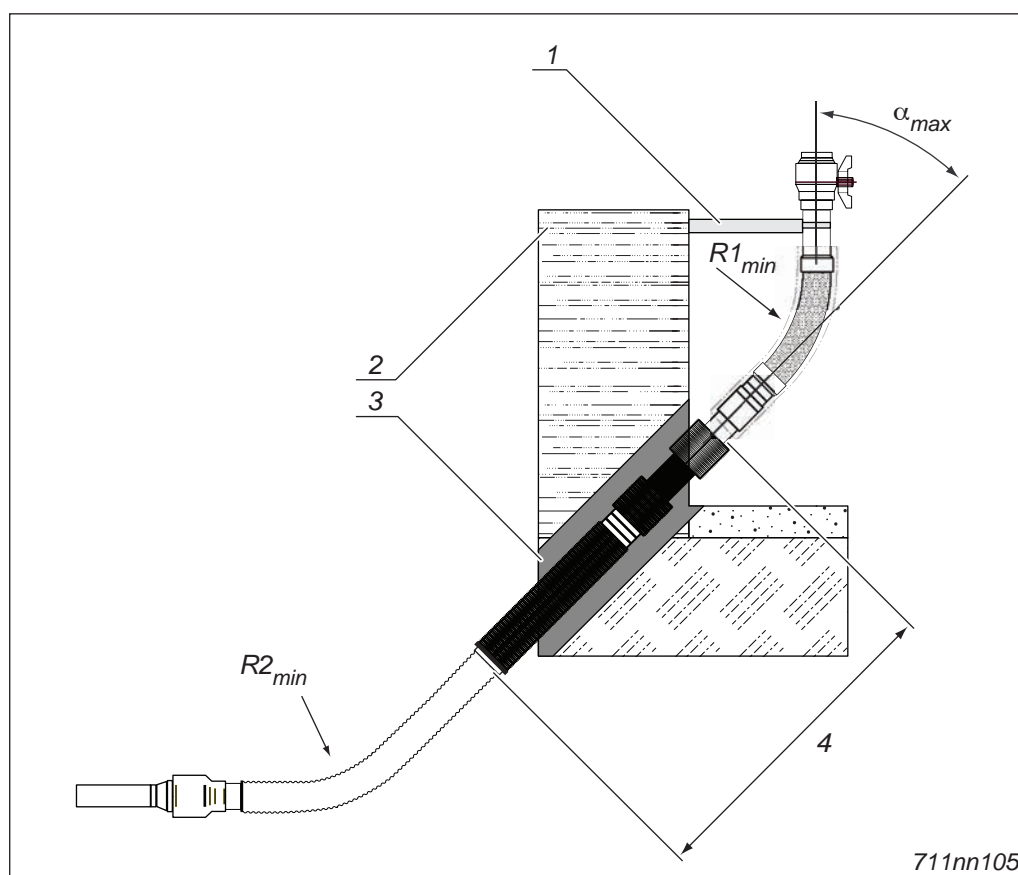
Fig. 4-5 DUO-FLEX / Innen-Flex
